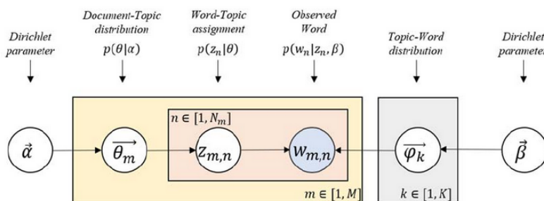
Gambar 2. Diagram Model LDA [25]
