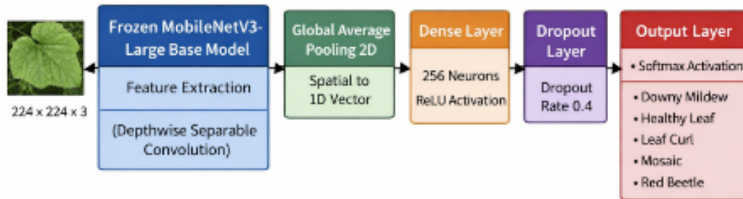
Gambar 4. Alur Pelatihan Model MobileNetV3-Large
