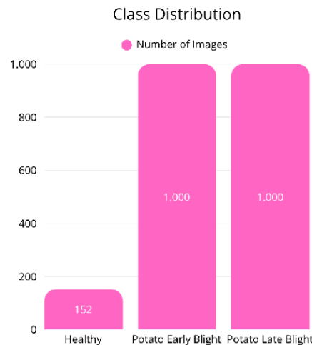
Figure 1. Class Distribution
