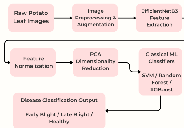
Figure 5. Architecture of the proposed hybrid deep feature learning
