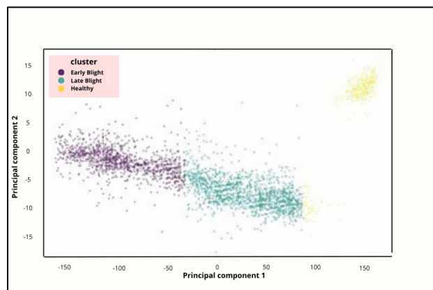
Figure 3. Cluster analysis (K-means) of tested dataset
