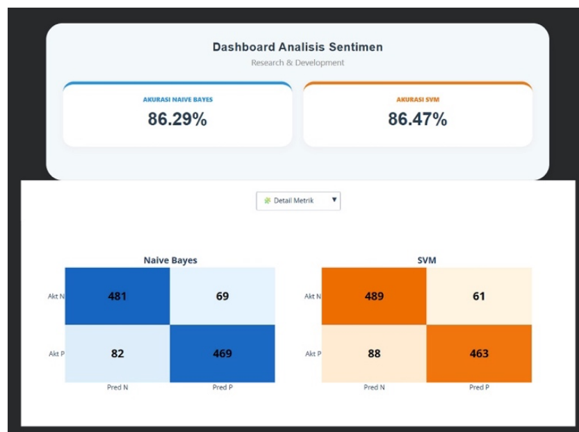
Gambar 2. Dashboard Analisis Sentimen Confusion Matrix
