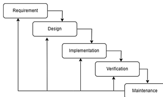
Gambar 2. Metode Waterfall
